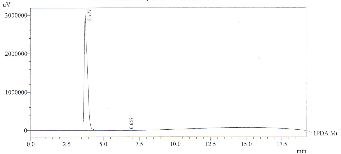
Chromatogram Harmaline D:\promonence\2010\Oct-10\091010C.lcd
